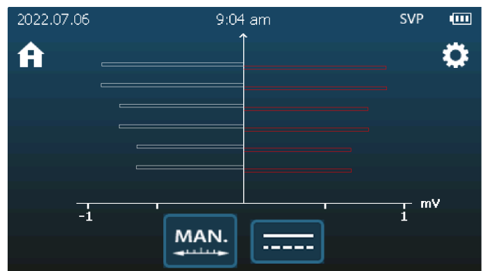
Sheath fault location with pulsed DC voltage
